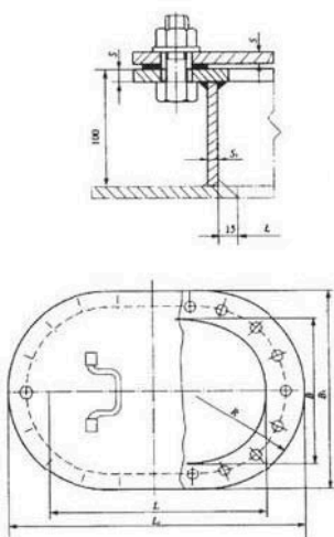
Marine manhole cover GB11628-1989
