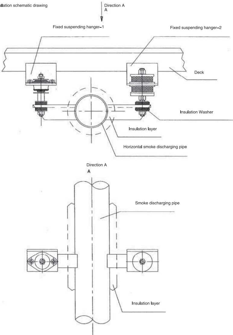
Installation schematic drawing
