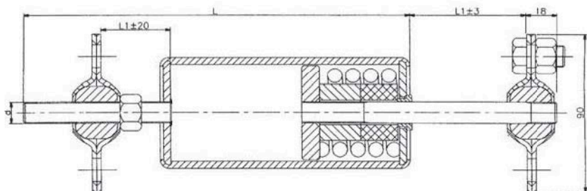
Fig.1. Metal spring hanger Type B (Outside color: Light yellow)
