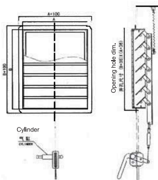
Type SQ (spring, pneumatic)
