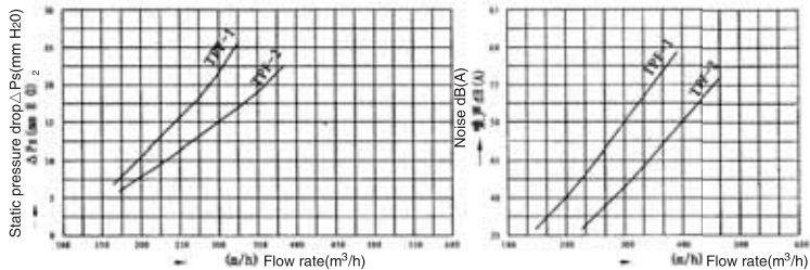
Performance chart
