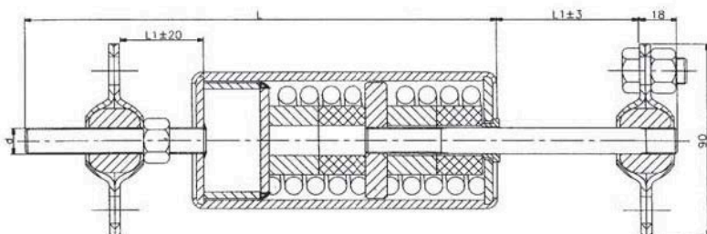
Fig.1. Metal spring hanger Type A (Outside color: Light green)
