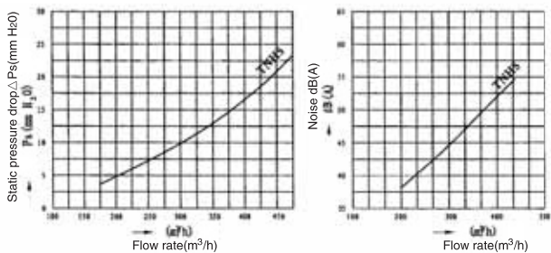
Performance chart
