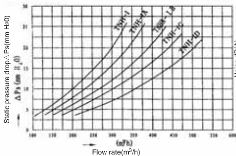
Performance chart
