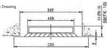
Outline Drawing
