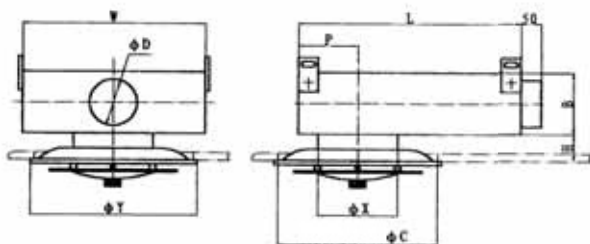
Ceiling opening \phi C
